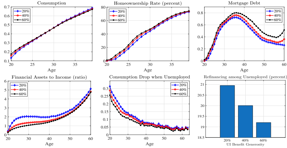
FIGURE B.3 – UI and Life-Cycle Dynamics
